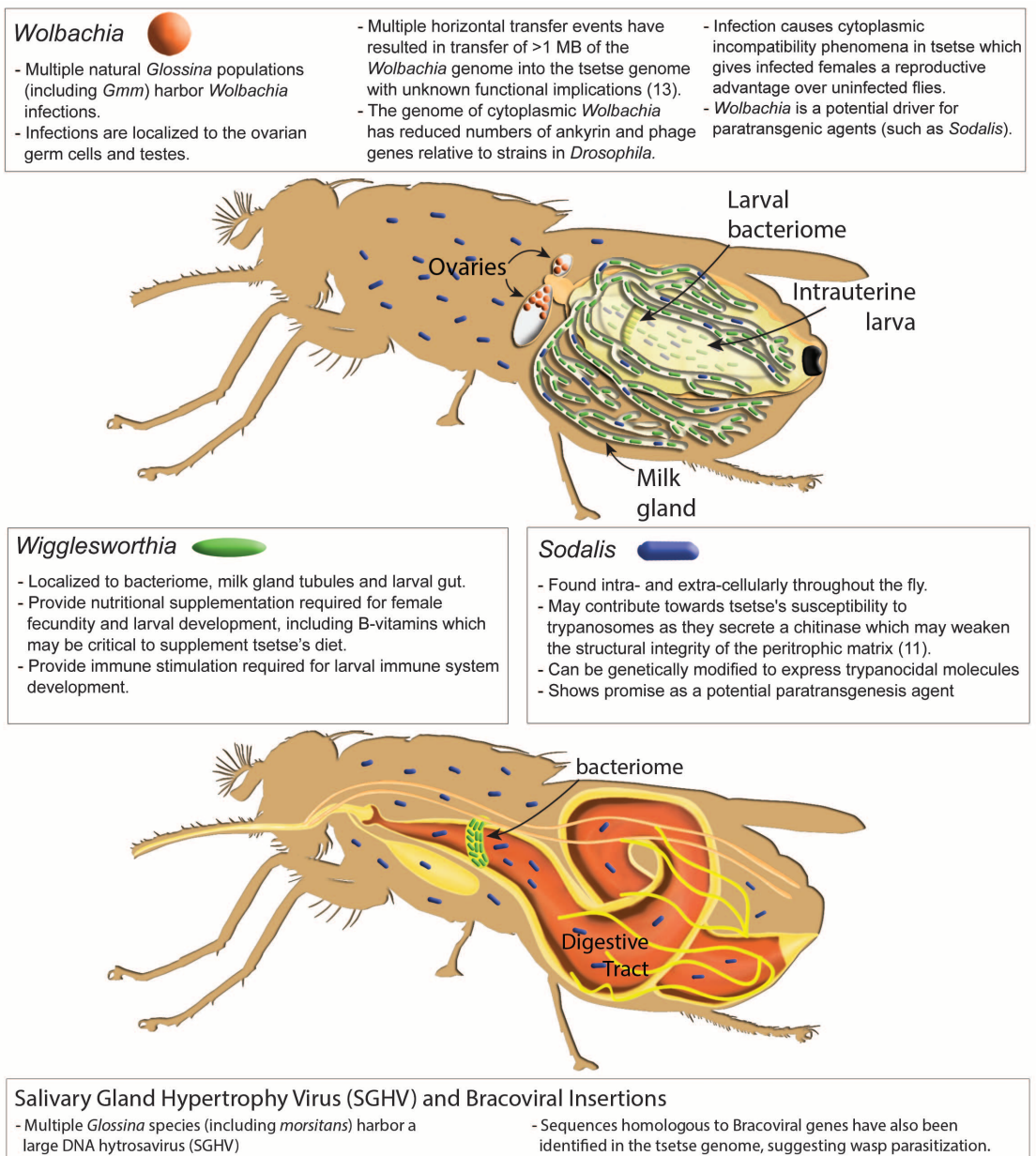
Fig. 2. Diagrammatic presentation of the Glossina microbiome, tissue localization of bacterial symbionts, physiological importance, and summary of genomic interactions. (Top) Glossina reproductive physiology and associated symbiont localizations. (Bottom) Glossina digestive physiology and the associated symbiont localizations. Associated text describes significant findings regarding the Glossina microbiome and the associated impacts in terms of Glossina immunity, nutrition, vectorial capacity, and vector control. Associated satellite references are listed within the figure as numbers in parentheses and correspond to the reference list (11, 13).
